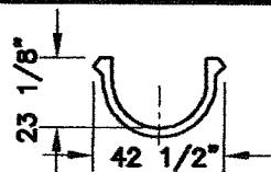
32" Open Flume
