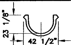
32" Open Flume
