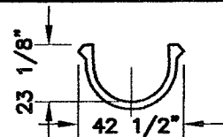
32" Open Flume
